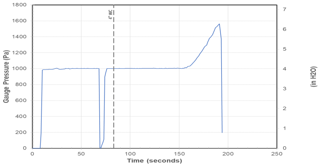
Figure 107. Gauge Pressure Data - Inlet
