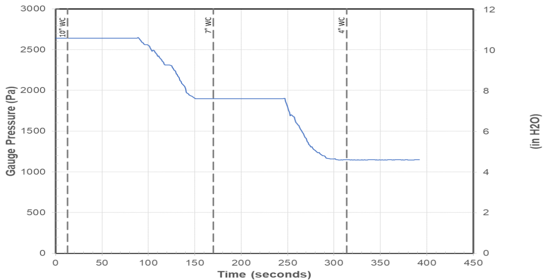
Figure 135. Gauge Pressure Data - Outlet
