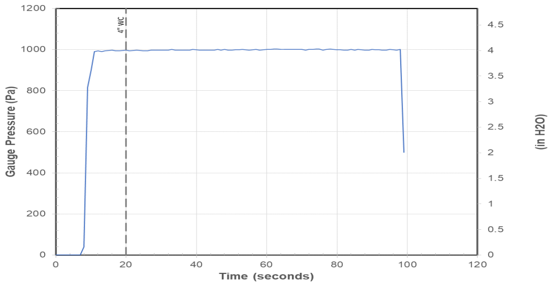
Figure 165. Gauge Pressure Data - Inlet
